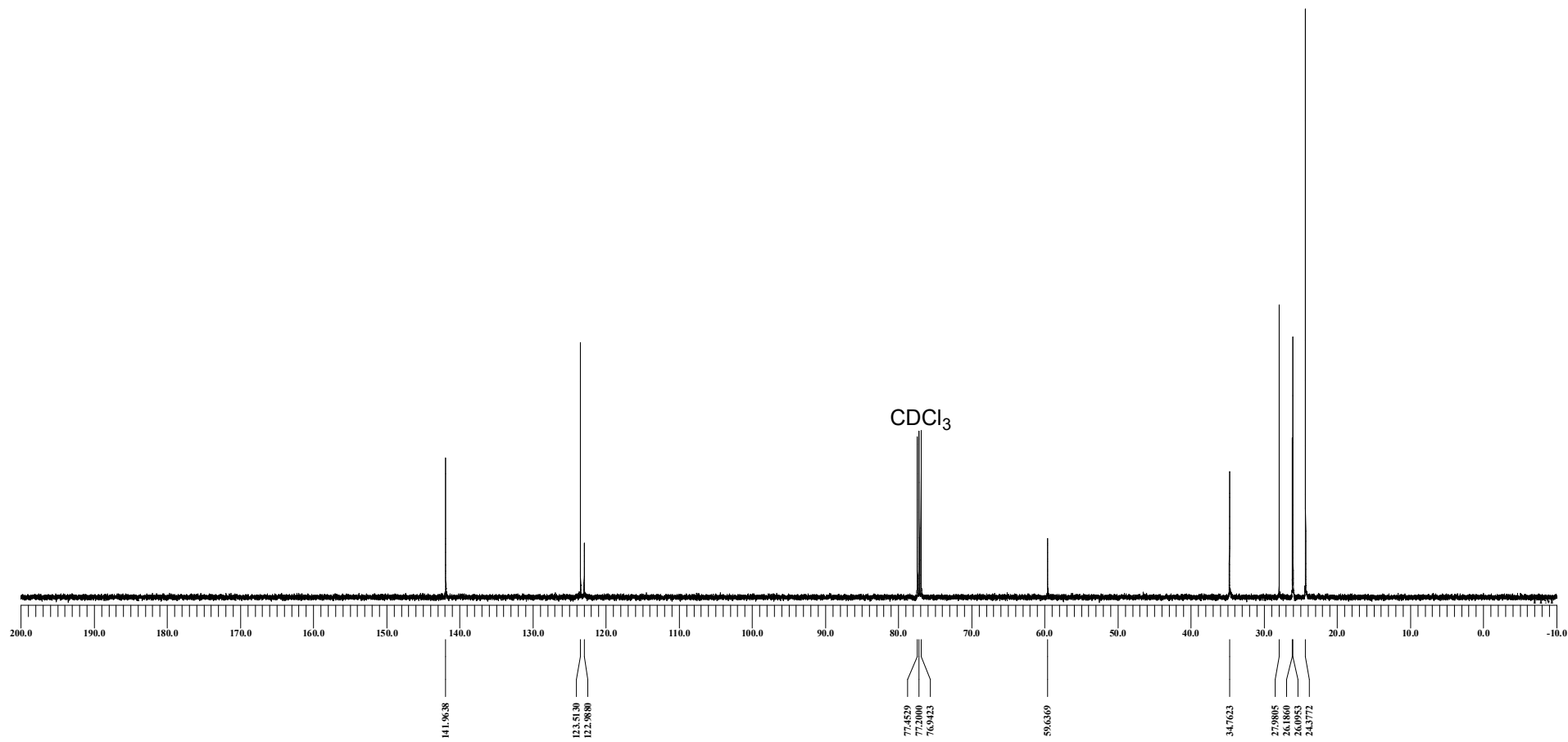
CyanH ( N -cyclohexyl-2,6-diisopropylaniline) ( 1 ) 13 C NMR (125 MHz, CDCl 3 )
