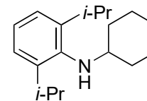
CyanH ( N -cyclohexyl-2,6-diisopropylaniline) ( 1 ) 13 C NMR (125 MHz, CDCl 3 )
